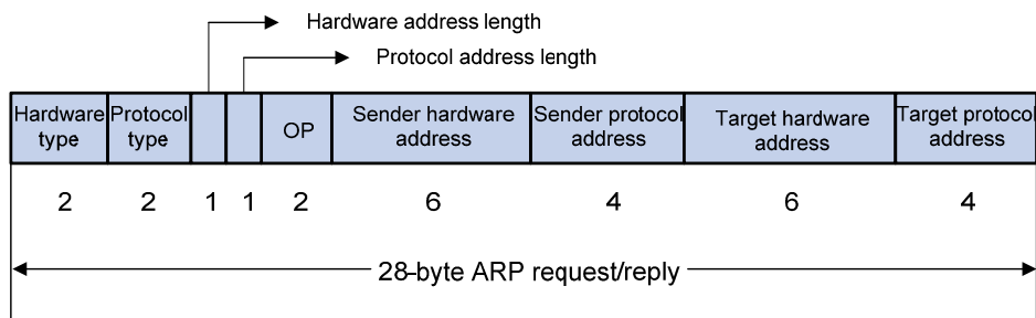
Figure 227 ARP message format
