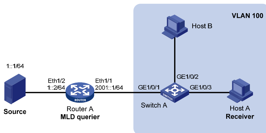
Figure 259 Network diagram
