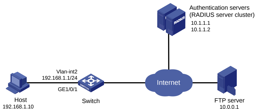
Figure 337 Network diagram
