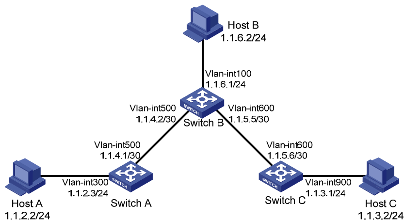
Figure 270 Network diagram
