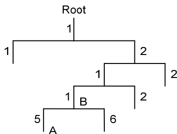
Figure 104 MIB tree
