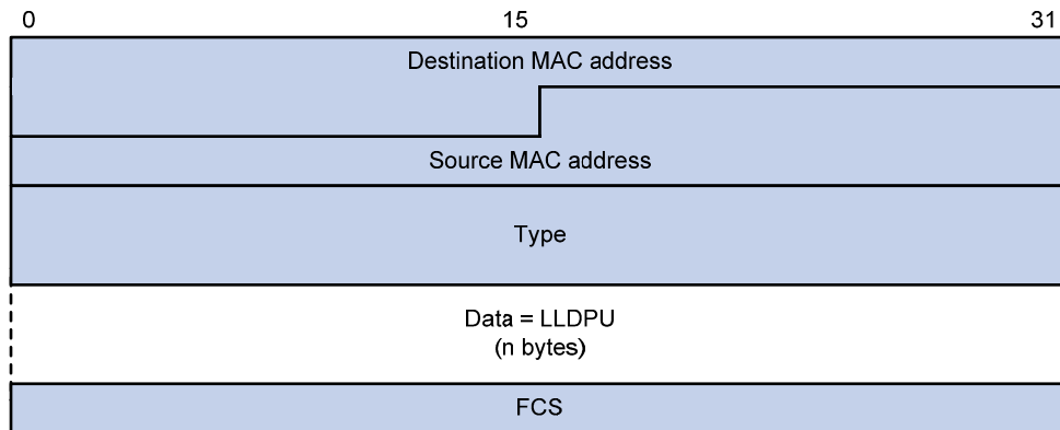
Figure 200 LLDPDU encapsulated in SNAP
