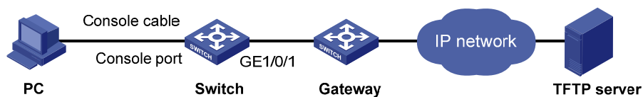
Figure 21 Network diagram
