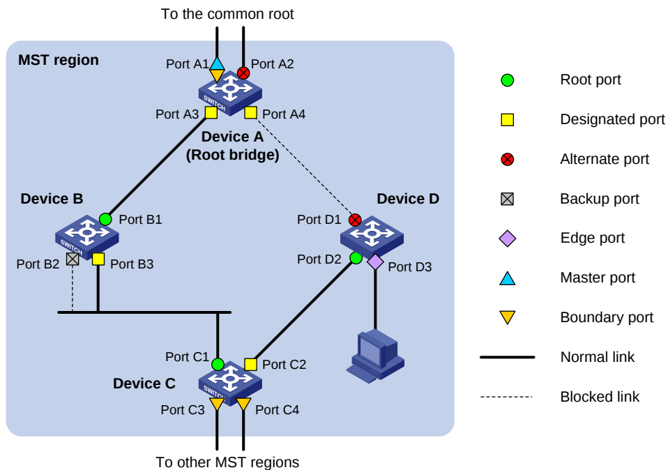
Figure 181 Port roles
