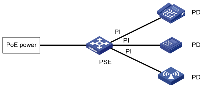
Figure 489 PoE system
