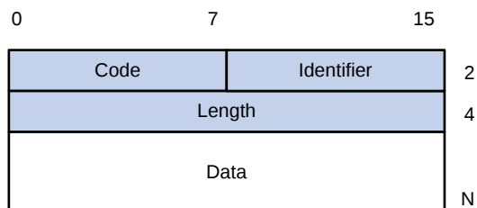
Figure 316 EAP packet format
