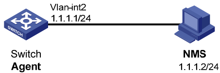
Figure 125 Network diagram
