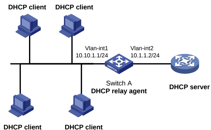
Figure 291 Network diagram
