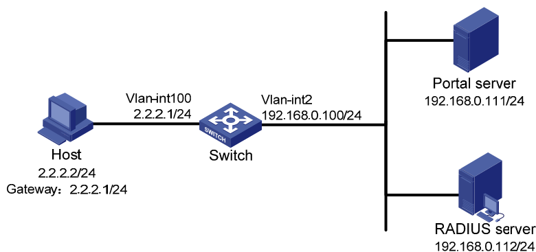
Figure 379 Network diagram
