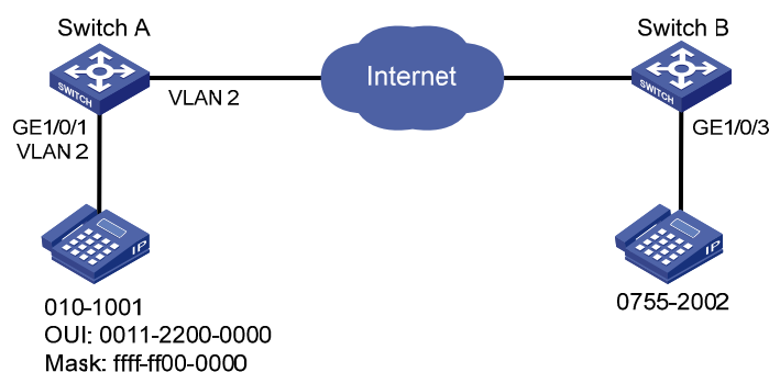
Figure 164 Network diagram
