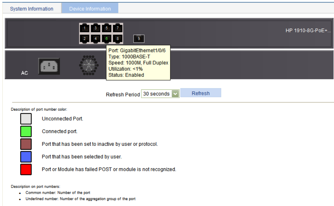
Figure 38 Device information
