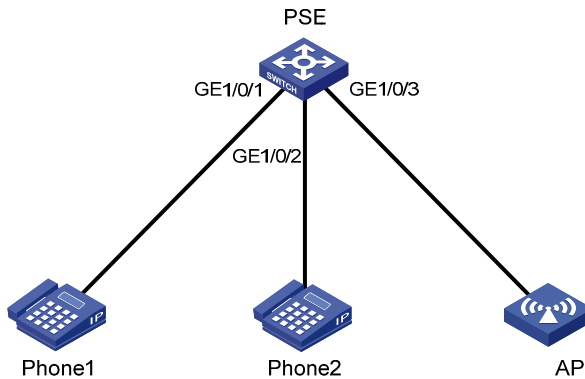
Figure 493 Network diagram
