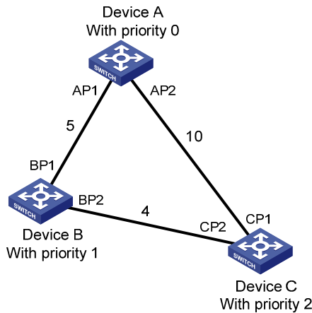
Figure 177 STP network
