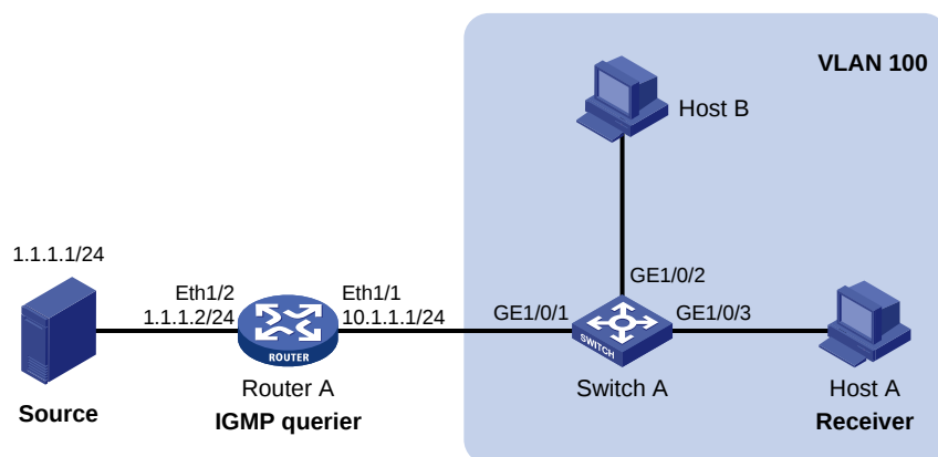
Figure 245 Network diagram
