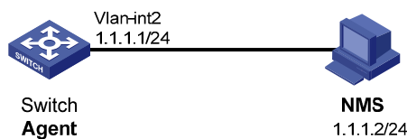
Figure 119 Network diagram
